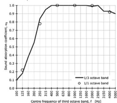
Mood AcuTex, pe 210g/m 2 , B1 Ecophon Master A 40 mm
